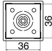
N51-24 BGA 35mm×35mm
