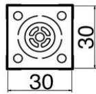
N51-23 BGA 29mm×29mm
